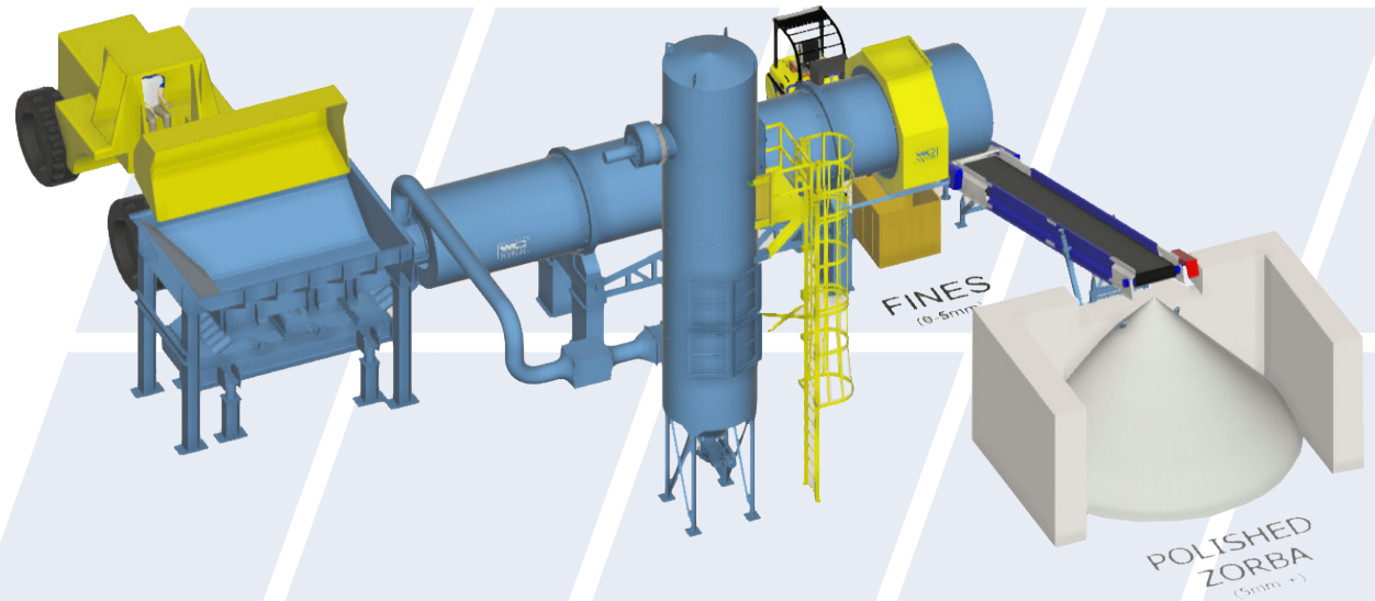
Batch Feeder CDC-40x16 with 10 Cubic Yard Hopper
